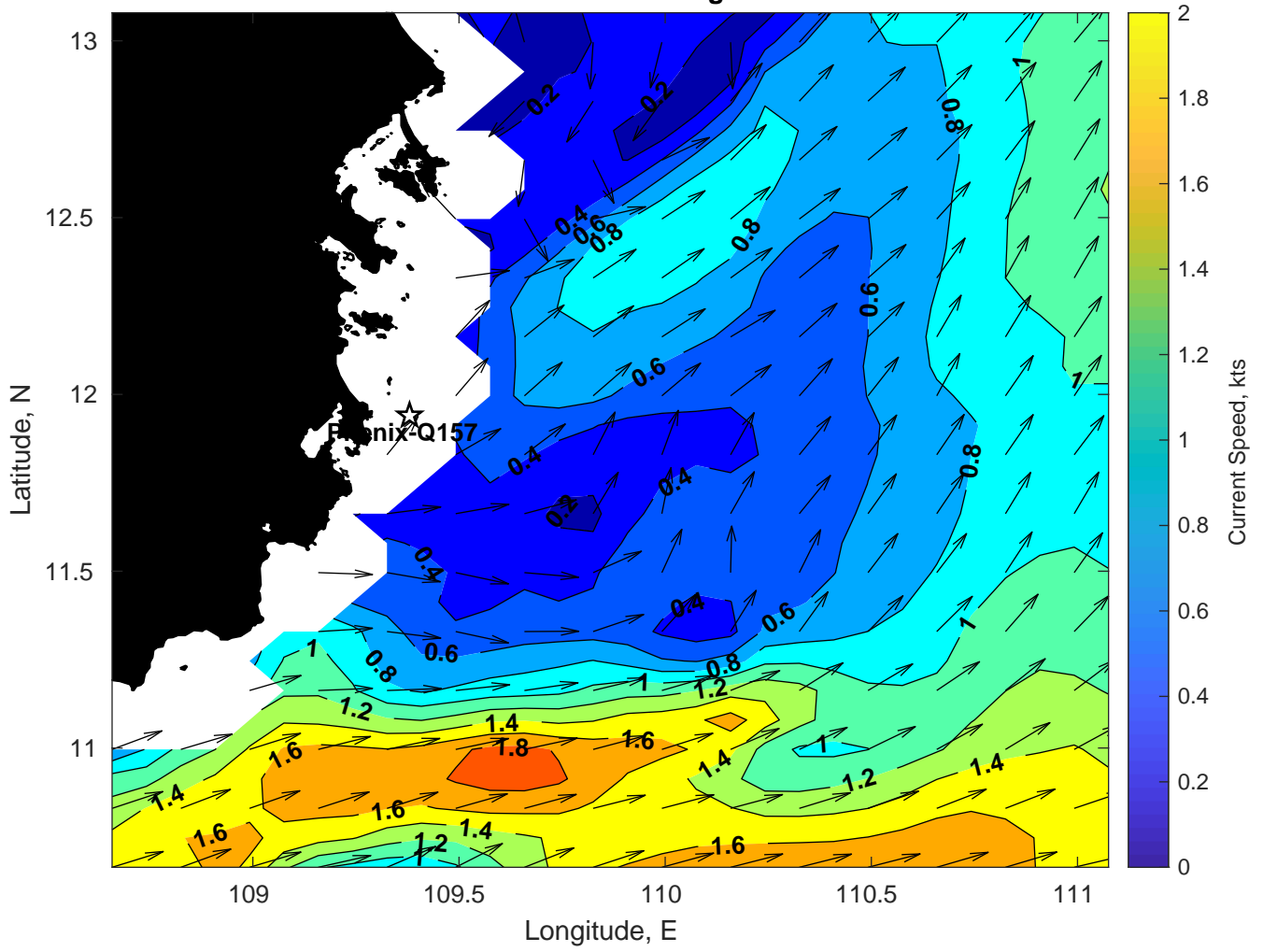
Surface Currents for Phenix-Q157 at 09-Aug-2024 00:00:00
