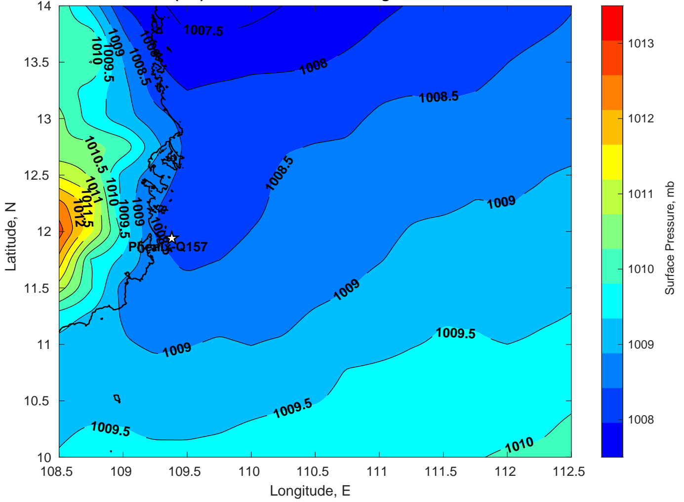
Surface Pressure (mb) for Phenix-Q157 at 09-Aug-2024 00:00:00
