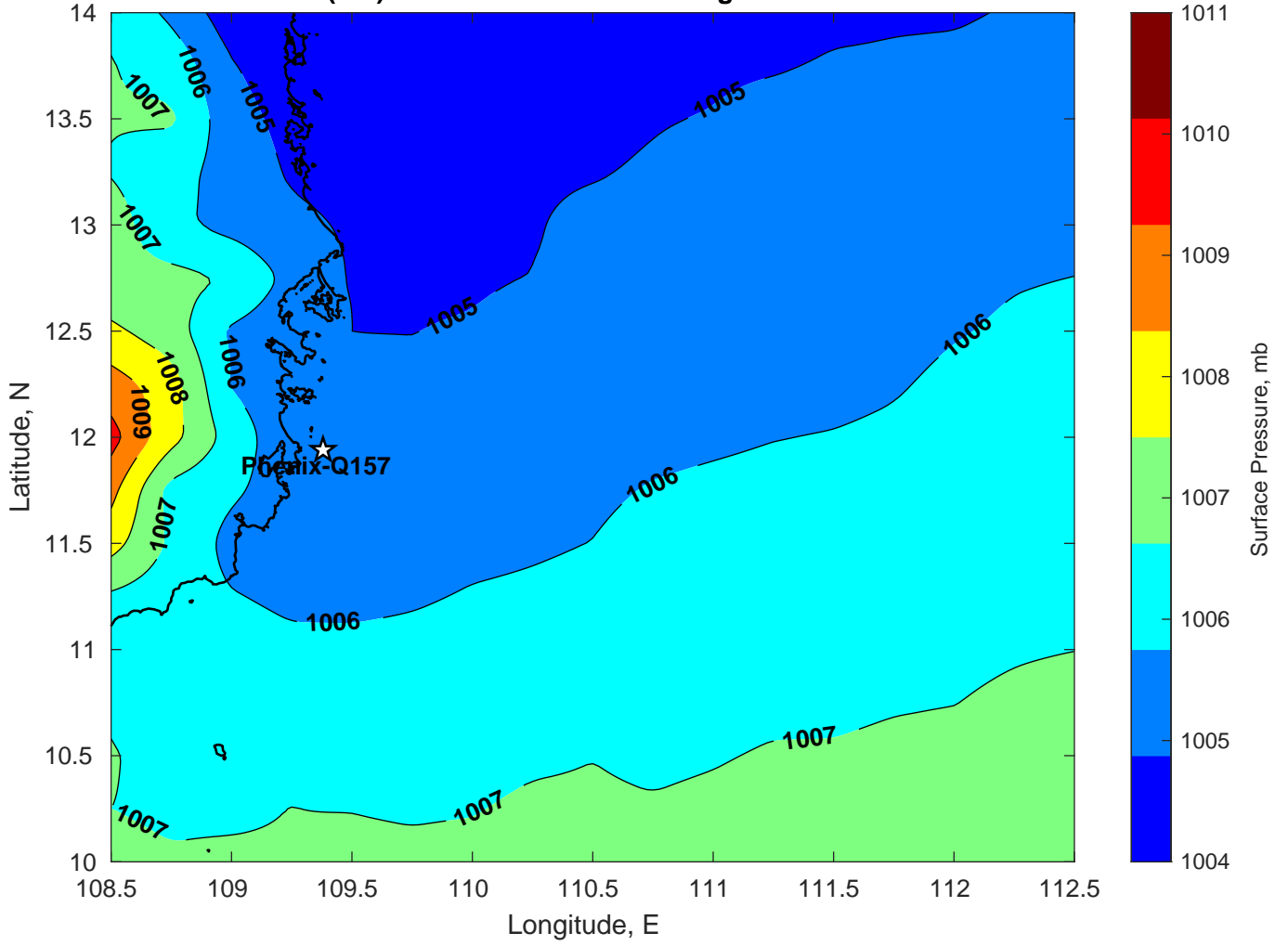
Surface Pressure (mb) for Phenix-Q157 at 11-Aug-2024 00:00:00
