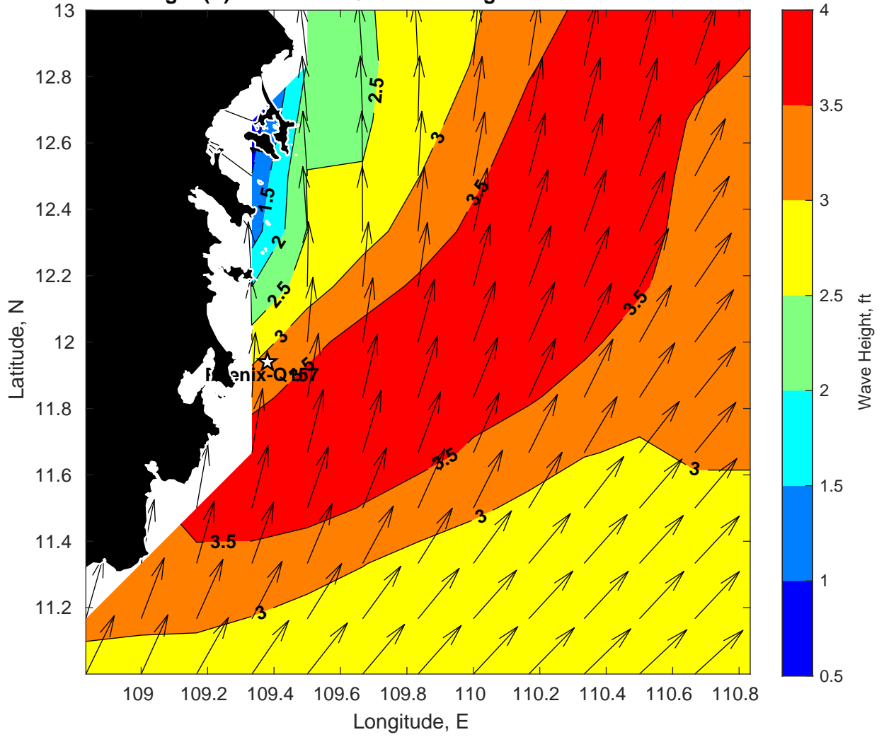
Wave Height (ft) for Phenix-Q157 at 09-Aug-2024 06:00:00
