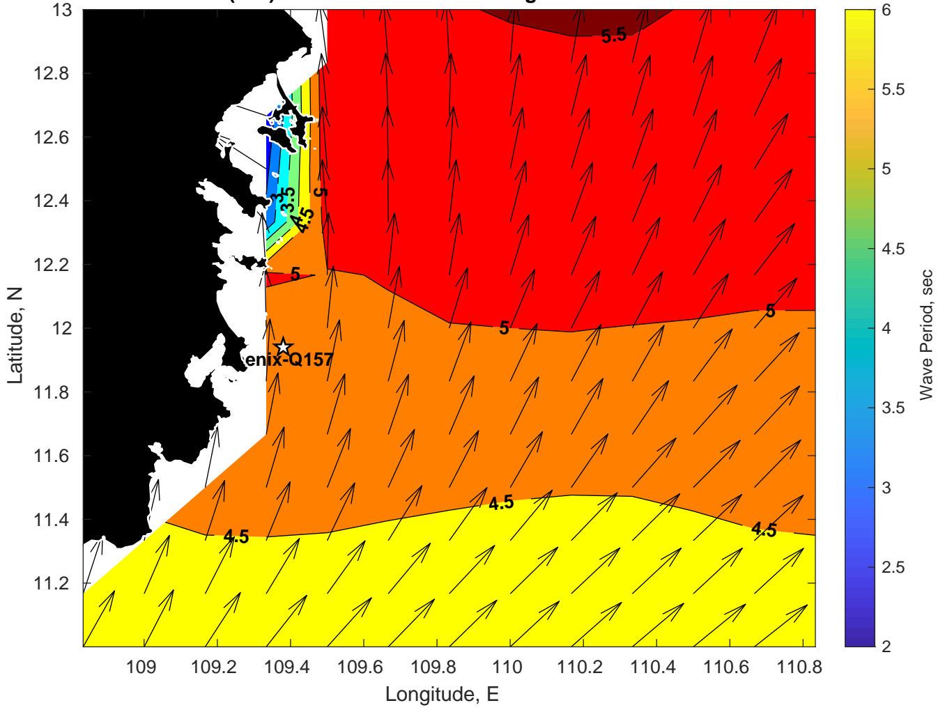
Wave Period (sec) for Phenix-Q157 at 09-Aug-2024 06:00:00
