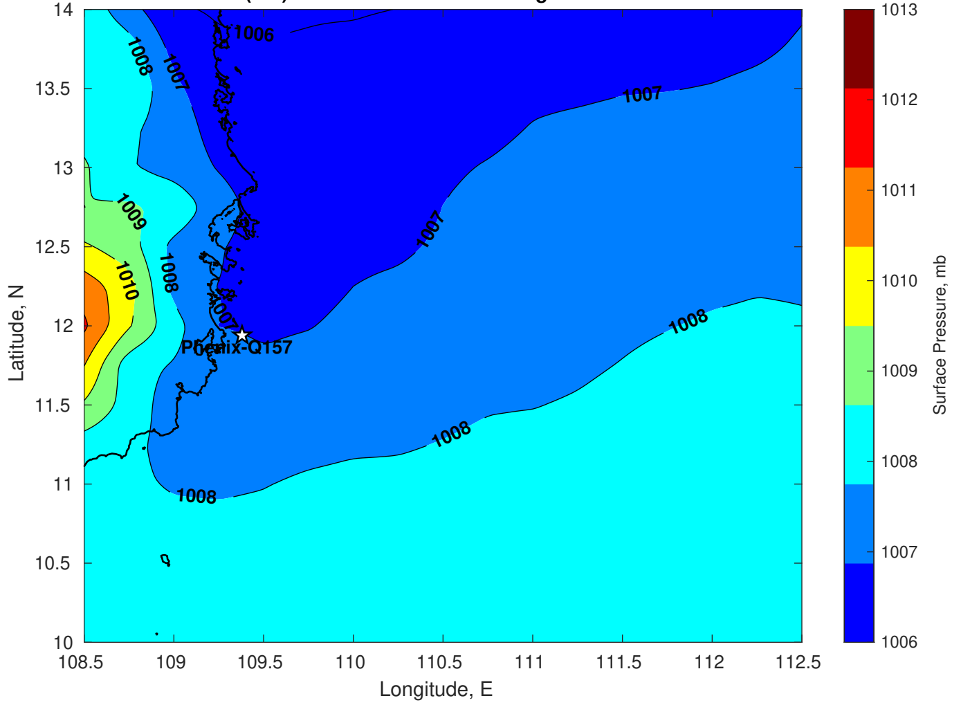
Surface Pressure (mb) for Phenix-Q157 at 10-Aug-2024 00:00:00
