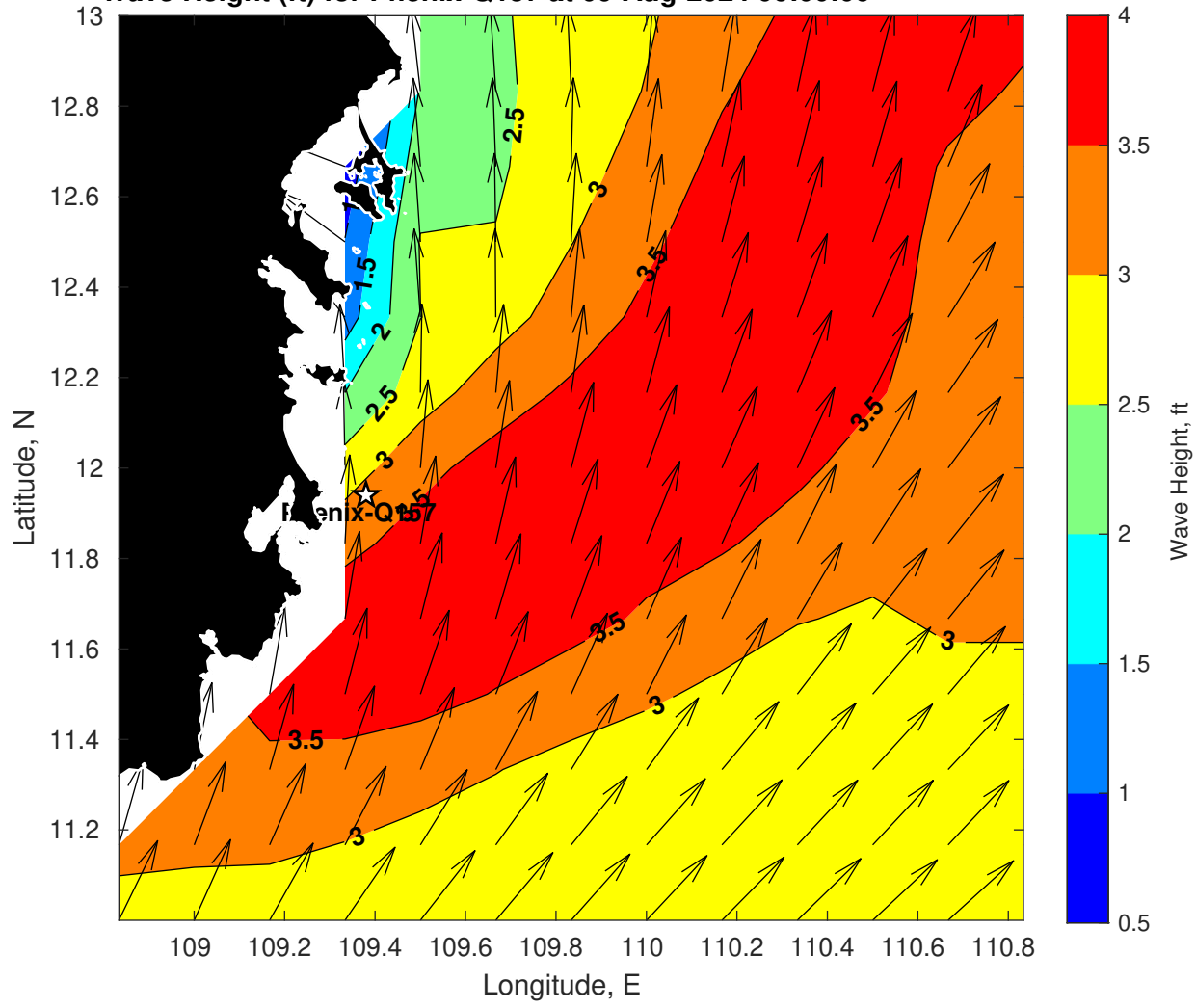
Wave Height (ft) for Phenix-Q157 at 09-Aug-2024 06:00:00
