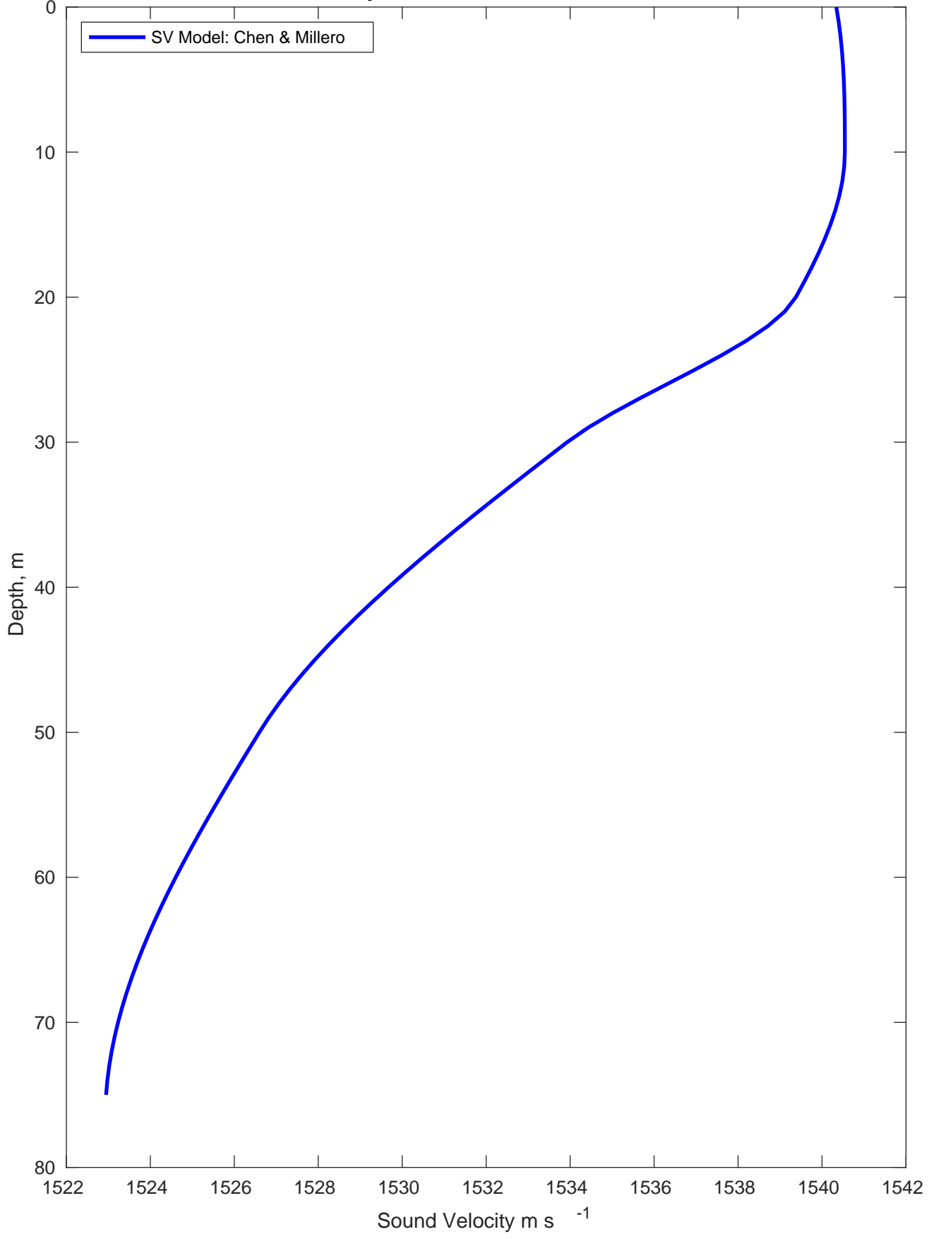
Sound Velocity Profile for Phenix-Q157 on 2
