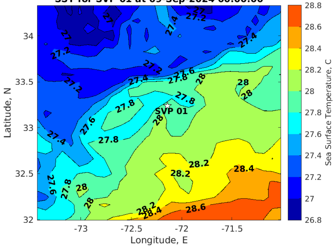
SST for SVP 01 at 09-Sep-2024 00:00:00
