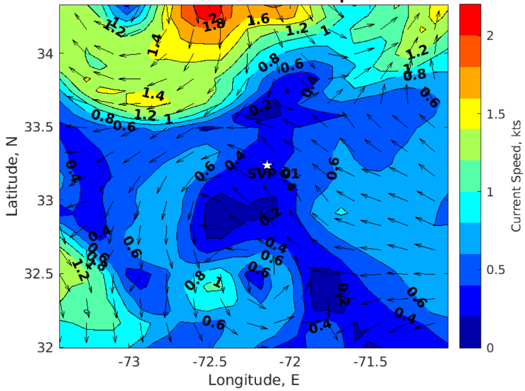
Surface Currents for SVP 01 at 09-Sep-2024 00:00:00
