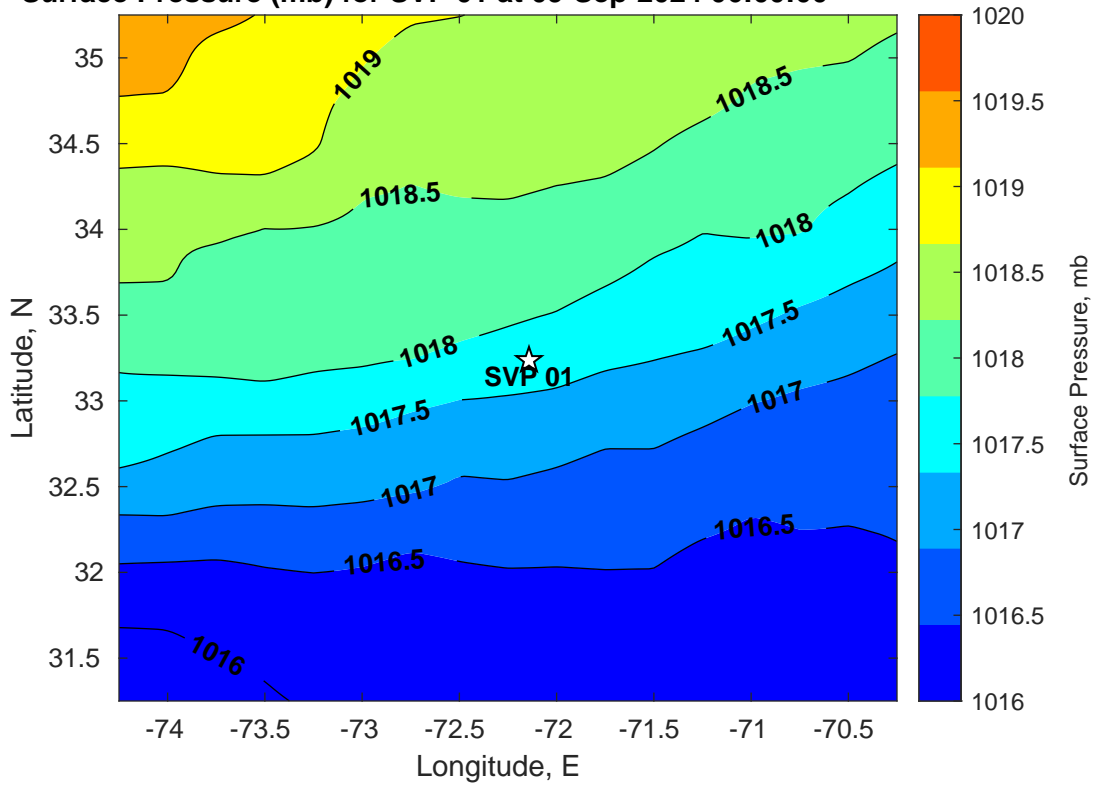
Surface Pressure (mb) for SVP 01 at 09-Sep-2024 06:00:00
