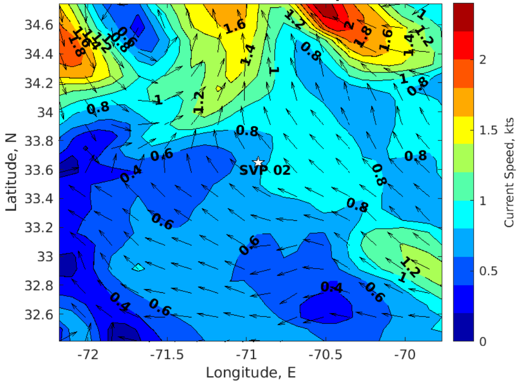
Surface Currents for SVP 02 at 09-Sep-2024 00:00:00
