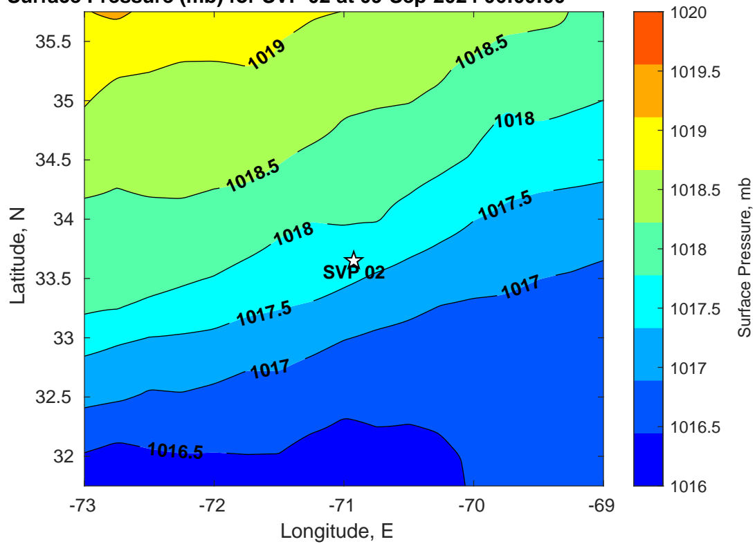
Surface Pressure (mb) for SVP 02 at 09-Sep-2024 06:00:00
