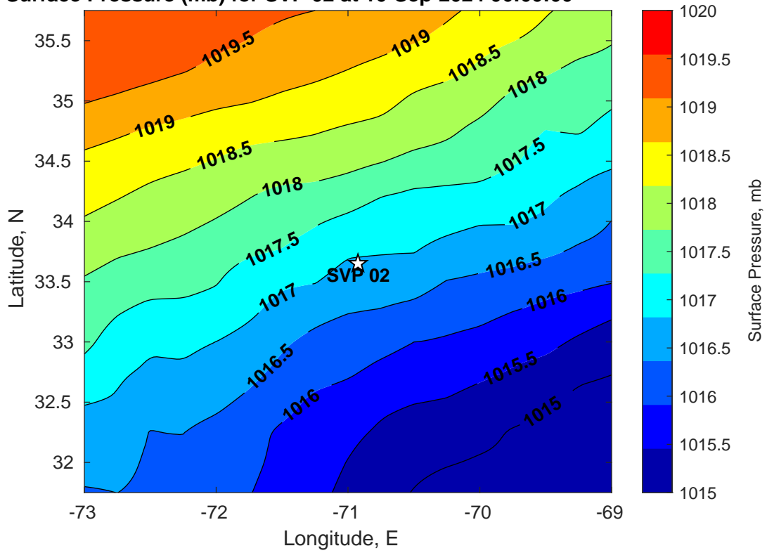
Surface Pressure (mb) for SVP 02 at 10-Sep-2024 06:00:00
