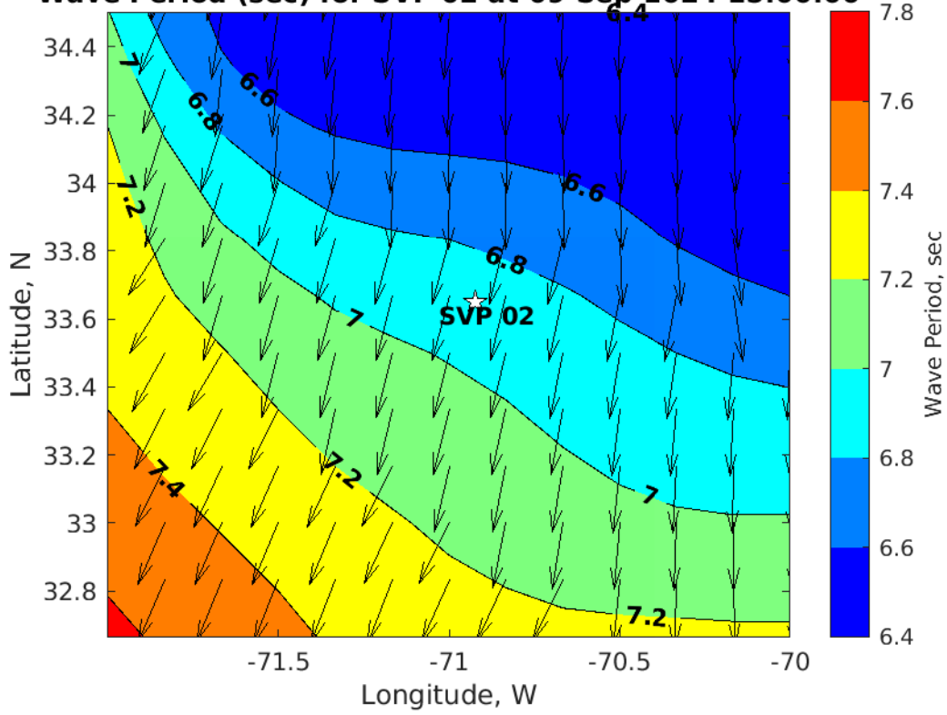
Wave Period (sec) for SVP 02 at 09-Sep-2024 15:00:00
