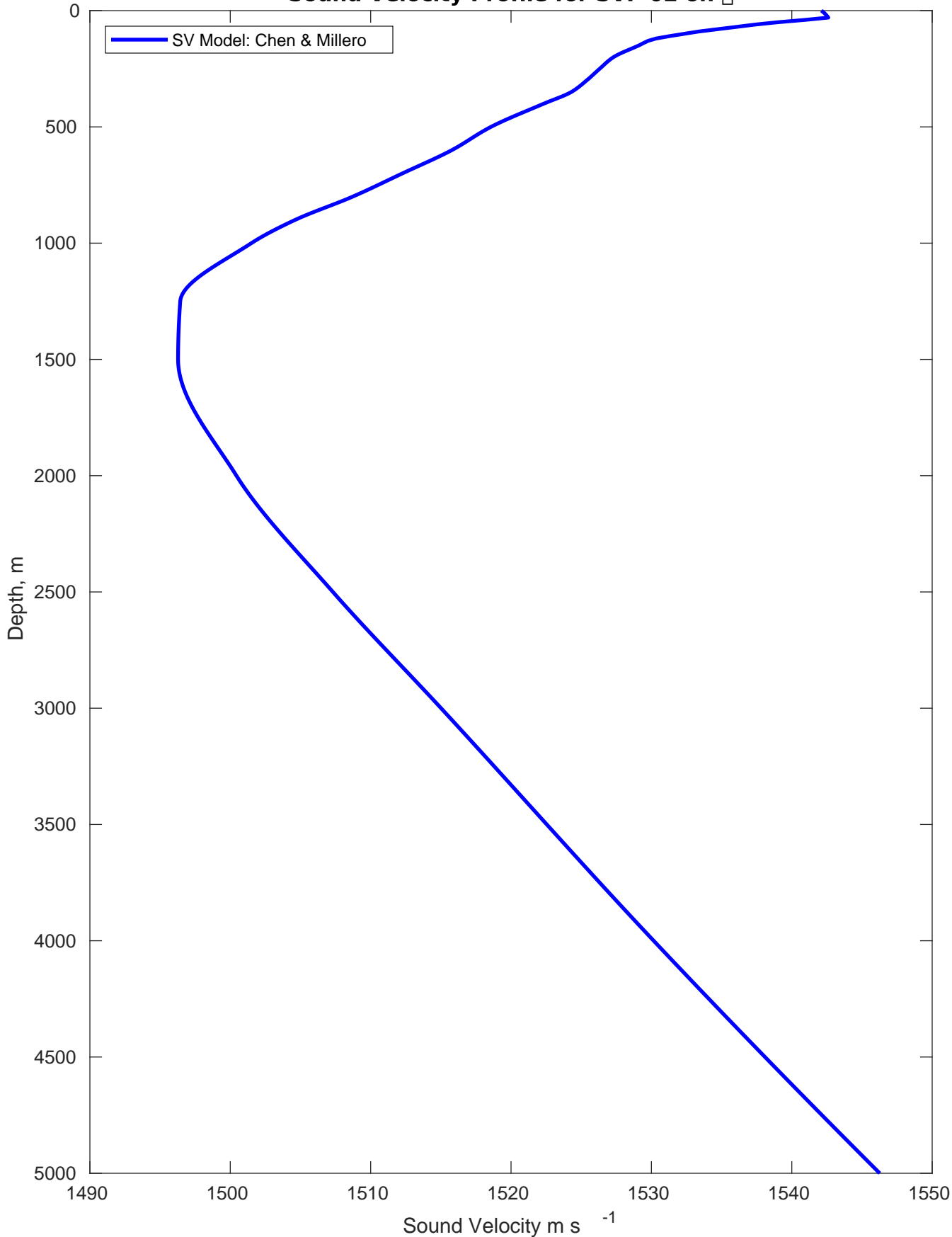
Sound Velocity Profile for SVP 02 on [ ]
