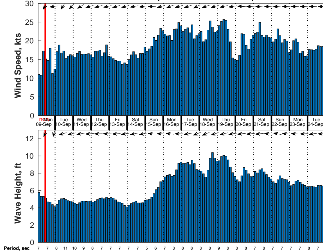
Wind & Wave Forecast for SVP 02 from 09-Sep-2024 01:00:00 to 25-Sep-2024 01:00:00
