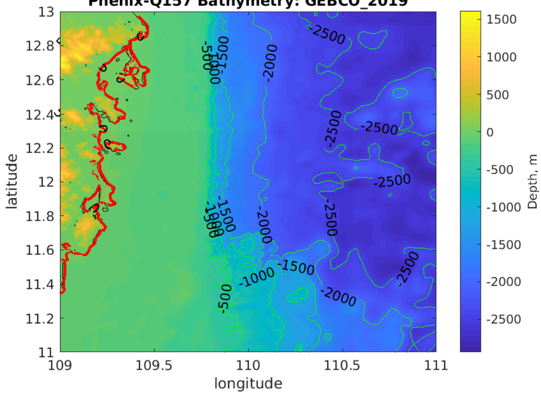
Phenix-Q157 Bathymetry: GEBCO_2019
