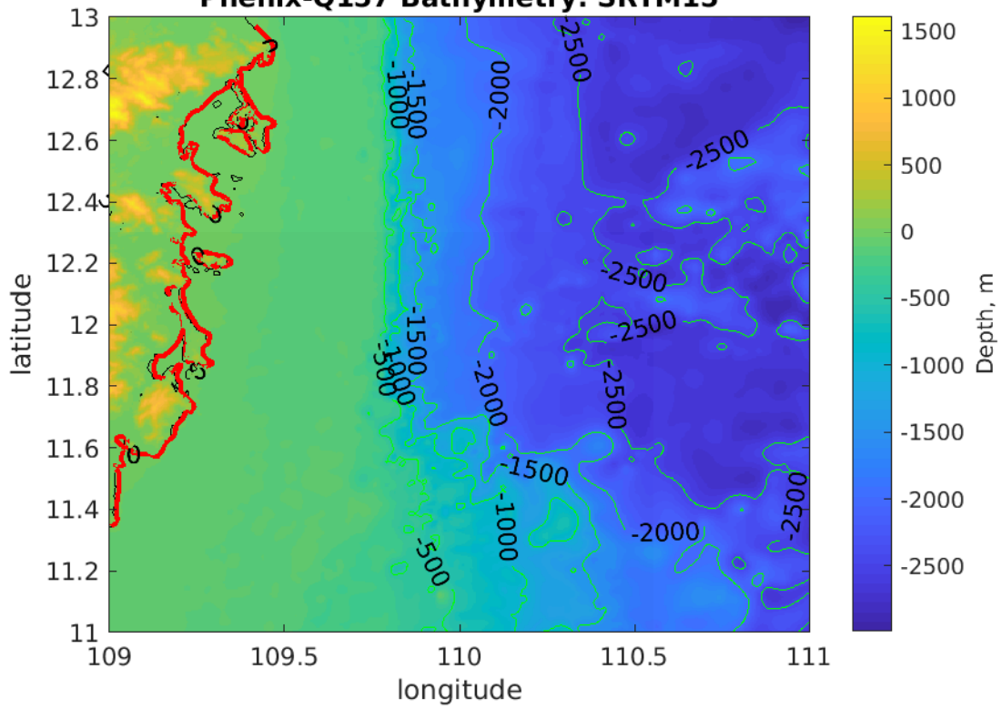
Phenix-Q157 Bathymetry: SRTM15
