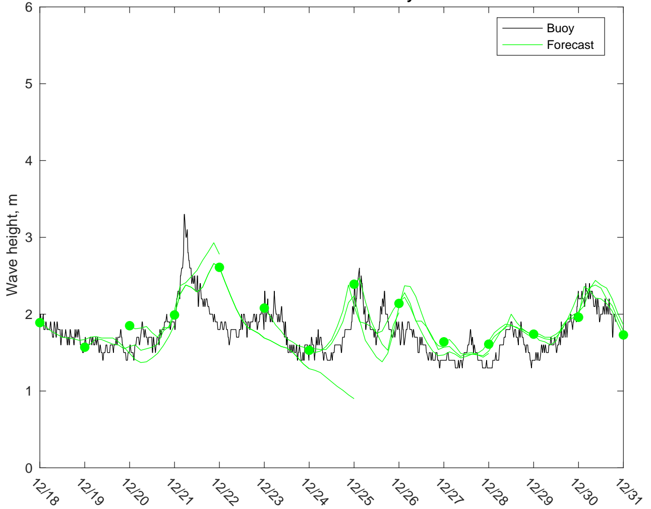
NDBC 41002 vs CMEMSWaves: 0 to 3 day forecast
