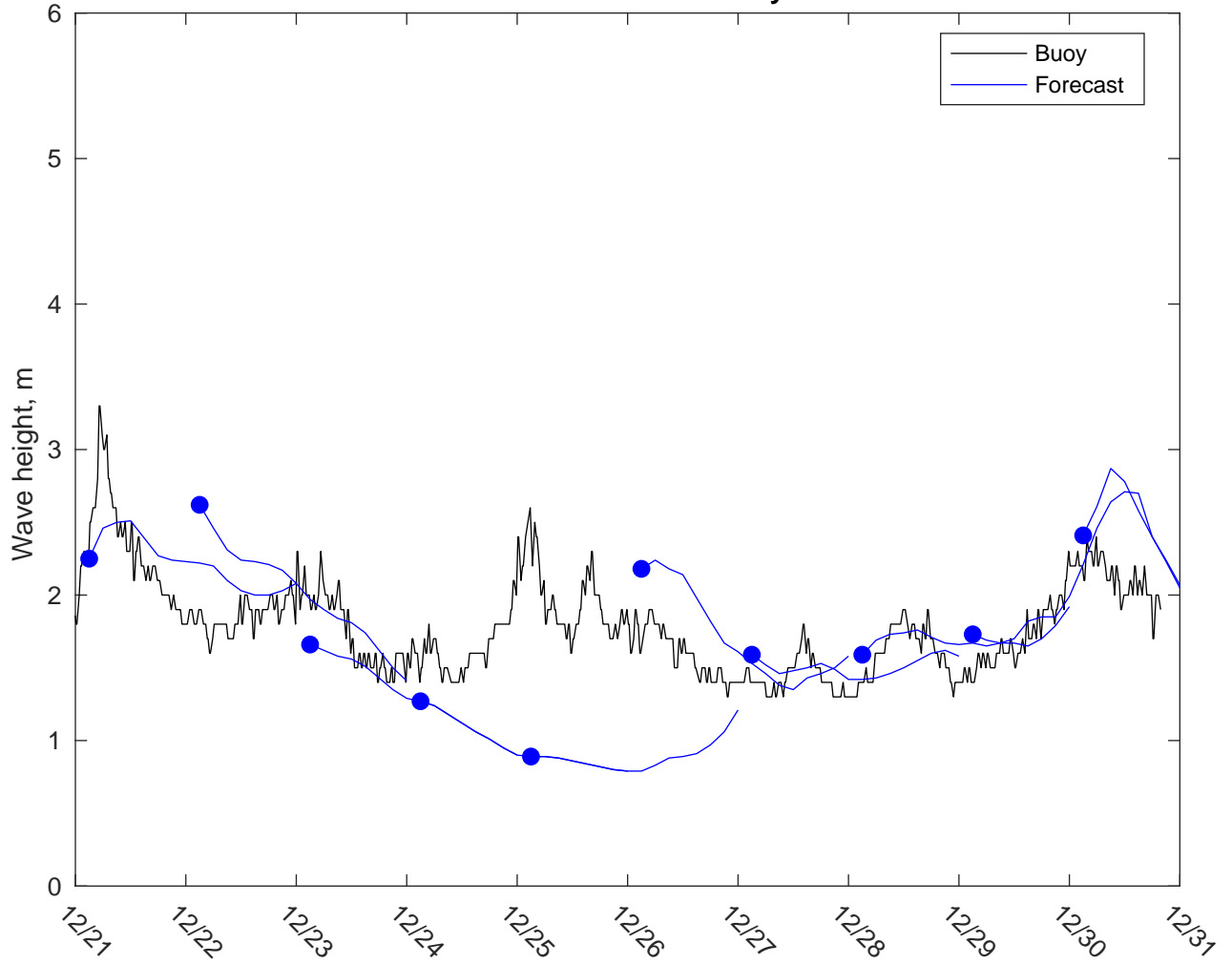
NDBC 41002 vs CMEMSWaves: 3 to 5 day forecast
