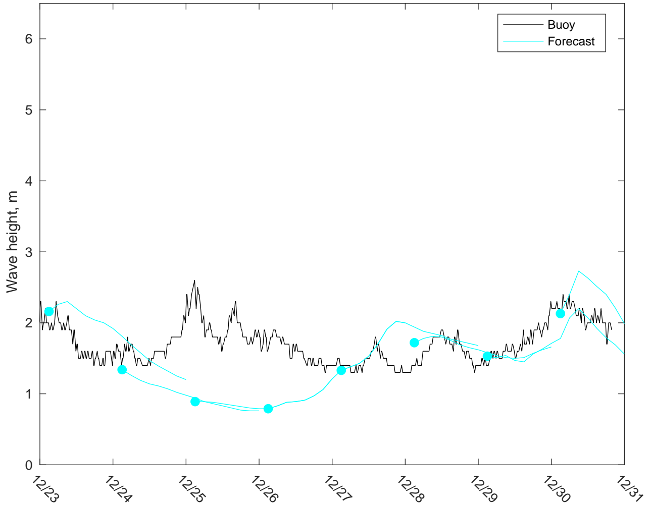
NDBC 41002 vs CMEMSWaves: 5 to 7 day forecast
