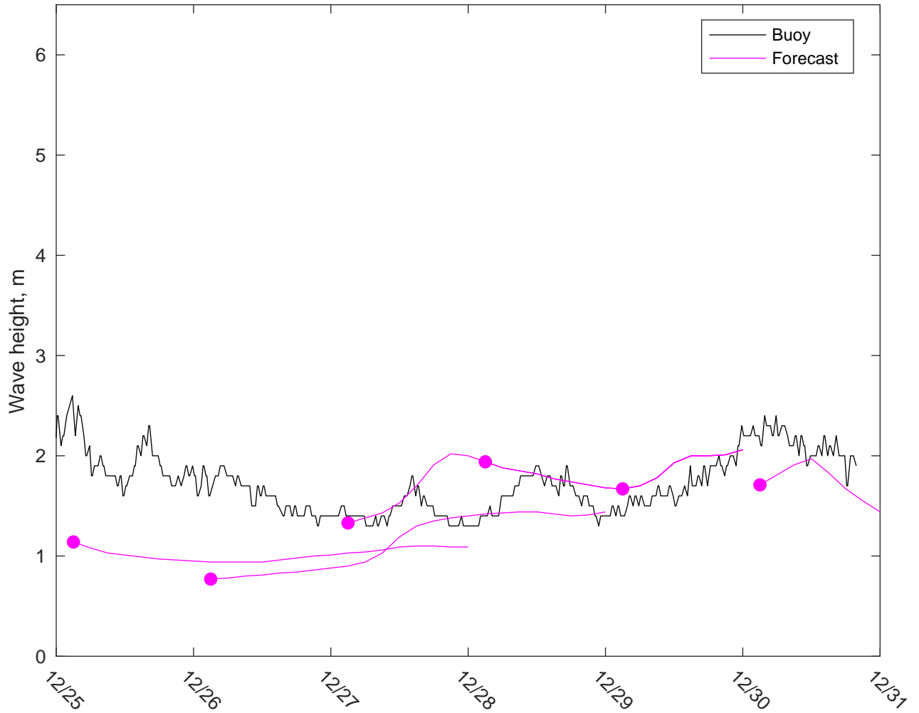
NDBC 41002 vs CMEMSWaves: 7 to 10 day forecast
