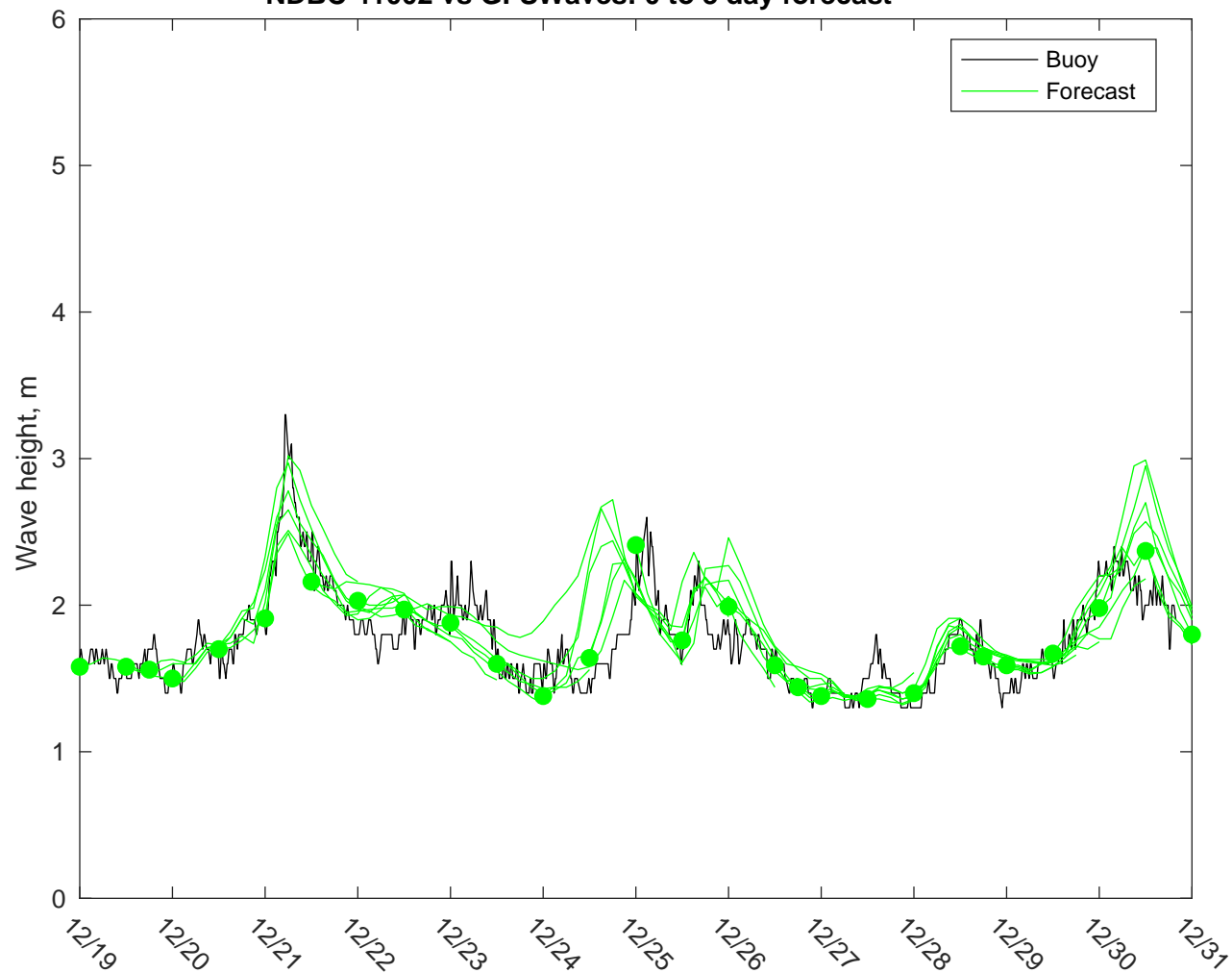
NDBC 41002 vs GFSWaves: 0 to 3 day forecast
