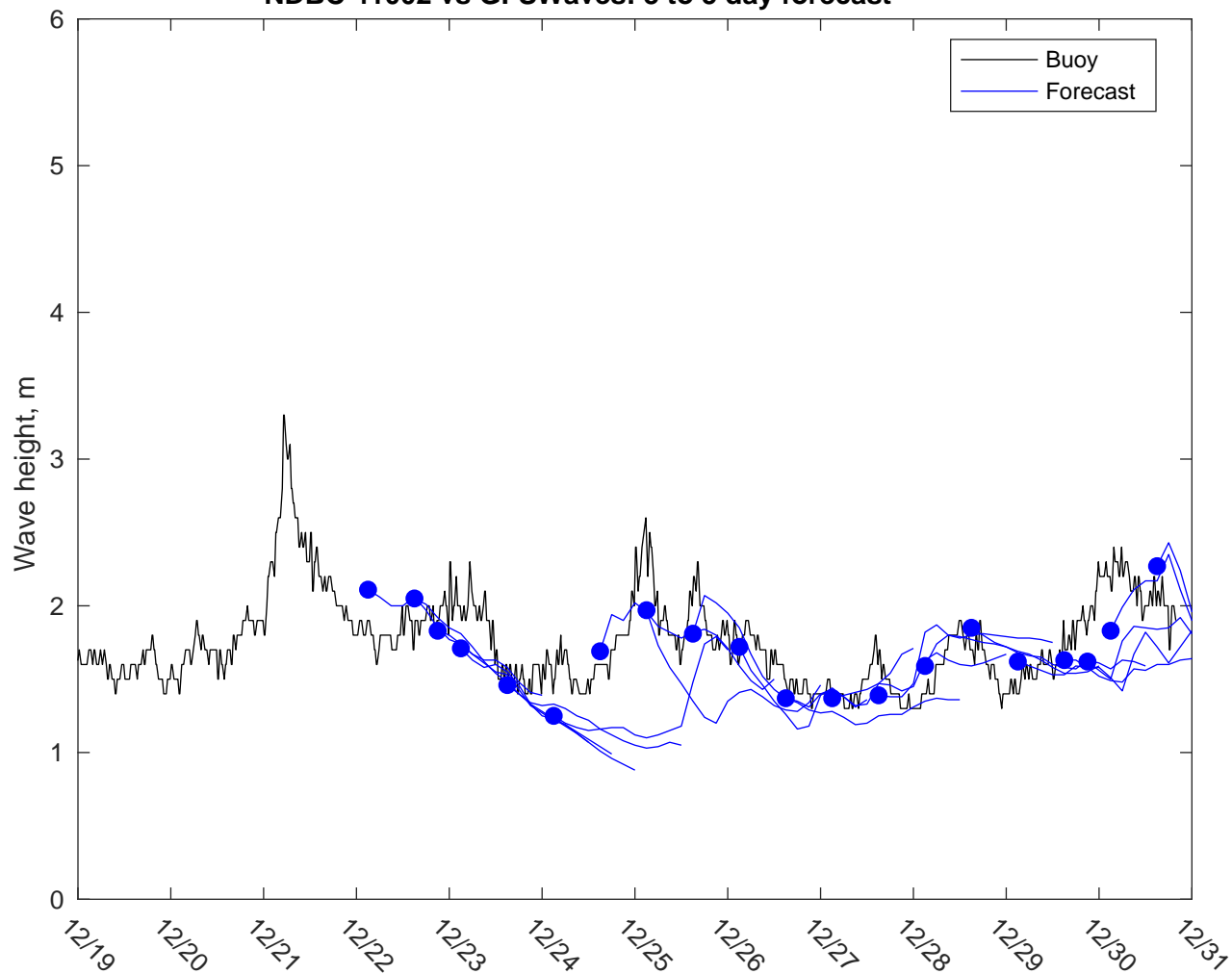
NDBC 41002 vs GFSWaves: 3 to 5 day forecast
