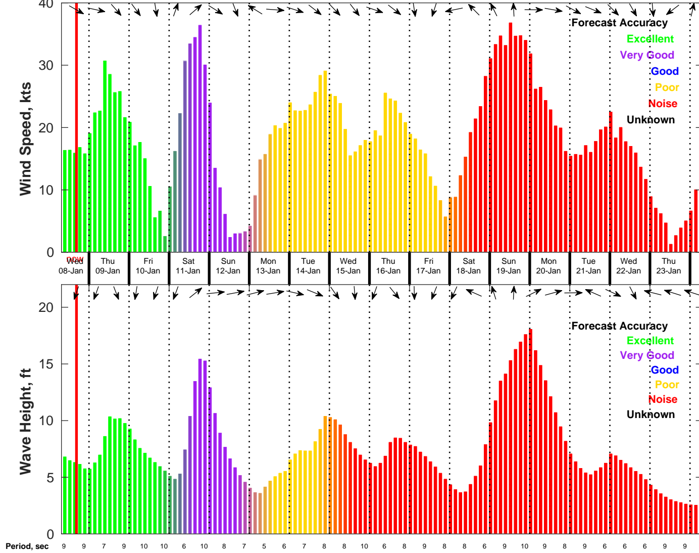
Wind & Wave Forecast for NDBC 41002 from 08-Jan-2025 08:00:00 to 24-Jan-2025 08:00:00
