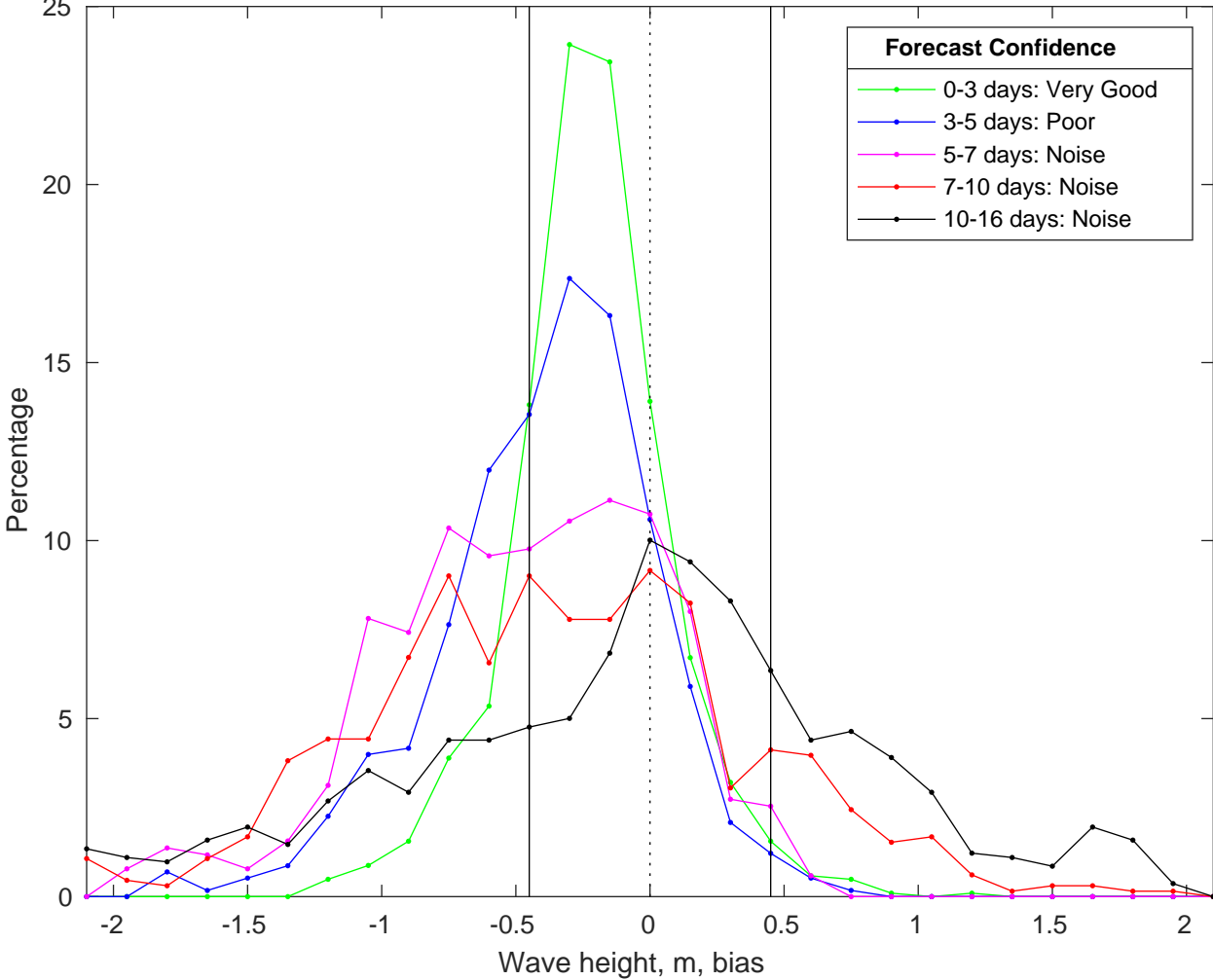
NDBC 41004 vs GFSWaves Bias Histogram: 08-Jan-2025
