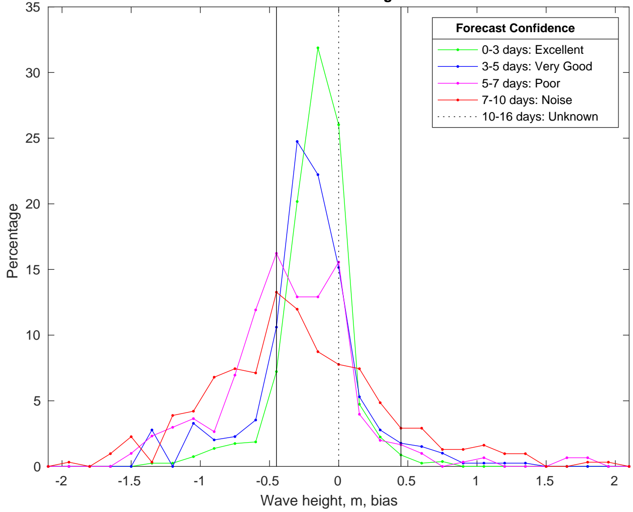
NDBC 41013 vs CMEMSWaves Bias Histogram: 08-Jan-2025
