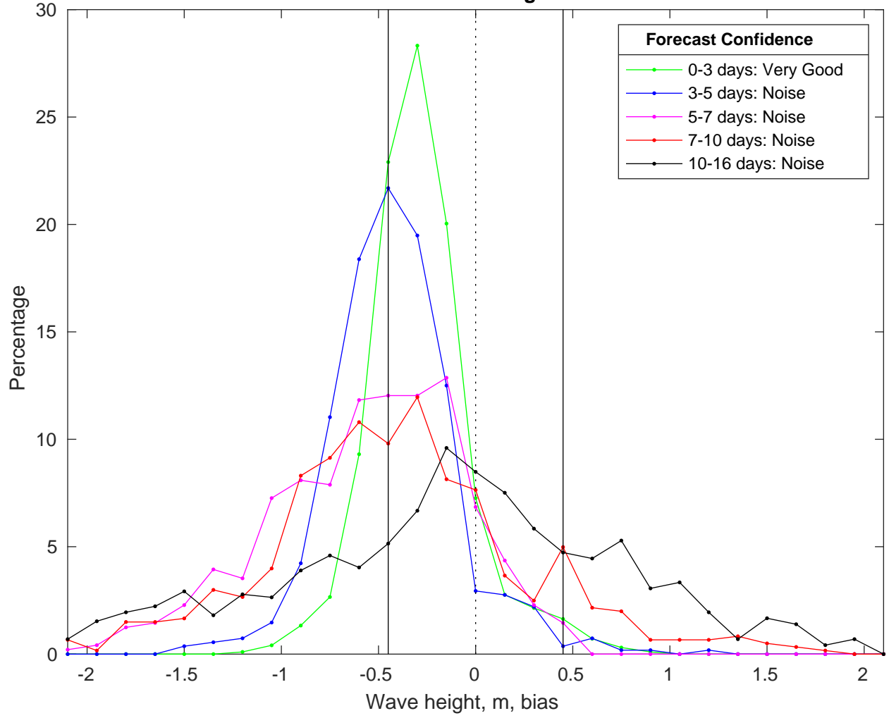
NDBC 41013 vs GFSWaves Bias Histogram: 08-Jan-2025
