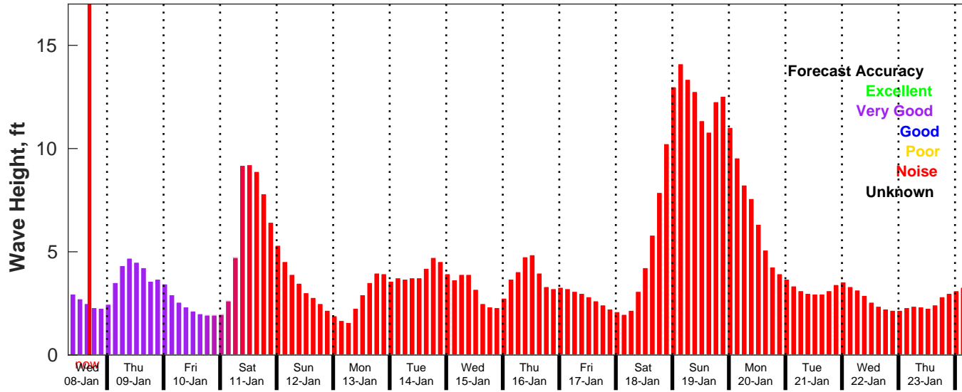
GFS Wave Forecast for NDBC 41013 from 08-Jan-2025 08:00:00 to 24-Jan-2025 08:00:00
