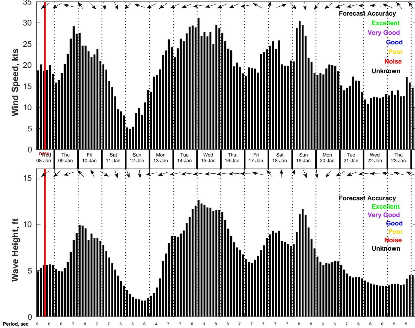
Wind & Wave Forecast for NDBC 42002 from 08-Jan-2025 06:00:00 to 24-Jan-2025 06:00:00
