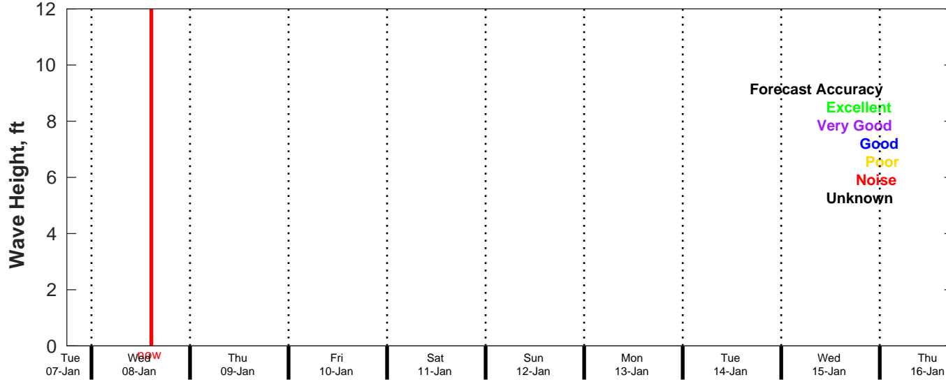
CMEMS Wave Forecast for NDBC 42020 from 07-Jan-2025 18:00:00 to 16-Jan-2025 18:00:00
