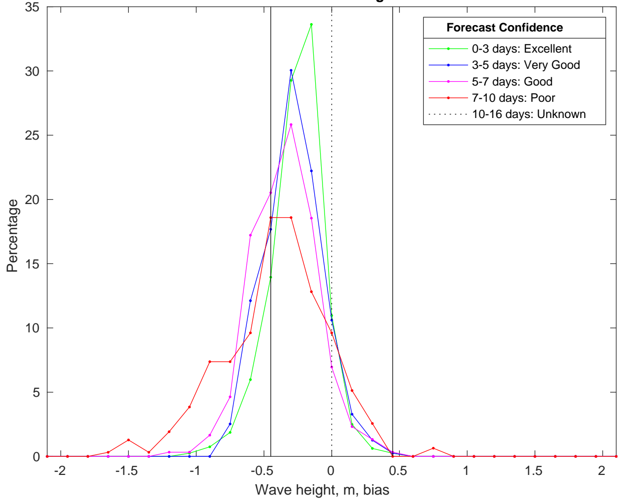
NDBC 42035 vs CMEMSWaves Bias Histogram: 08-Jan-2025
