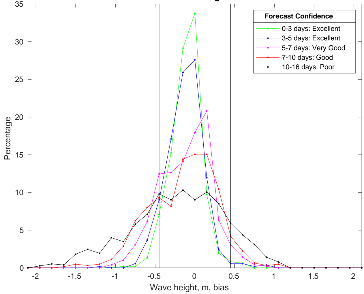
NDBC 42035 vs GFSWaves Bias Histogram: 08-Jan-2025
