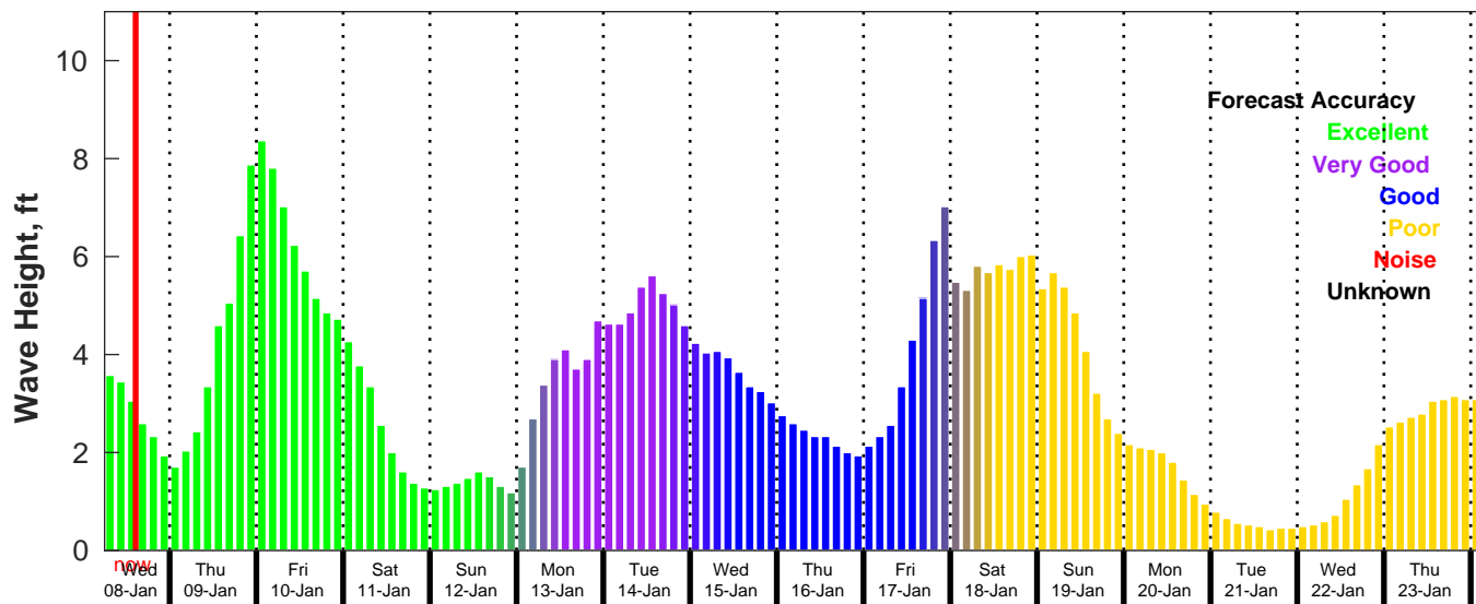
GFS Wave Forecast for NDBC 42035 from 08-Jan-2025 06:00:00 to 24-Jan-2025 06:00:00
