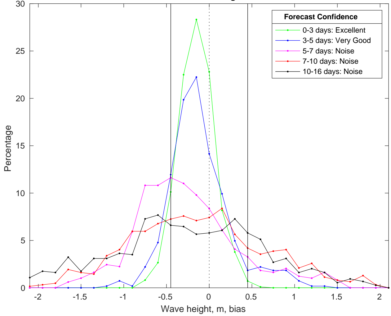
NDBC 42036 vs GFSWaves Bias Histogram: 08-Jan-2025
