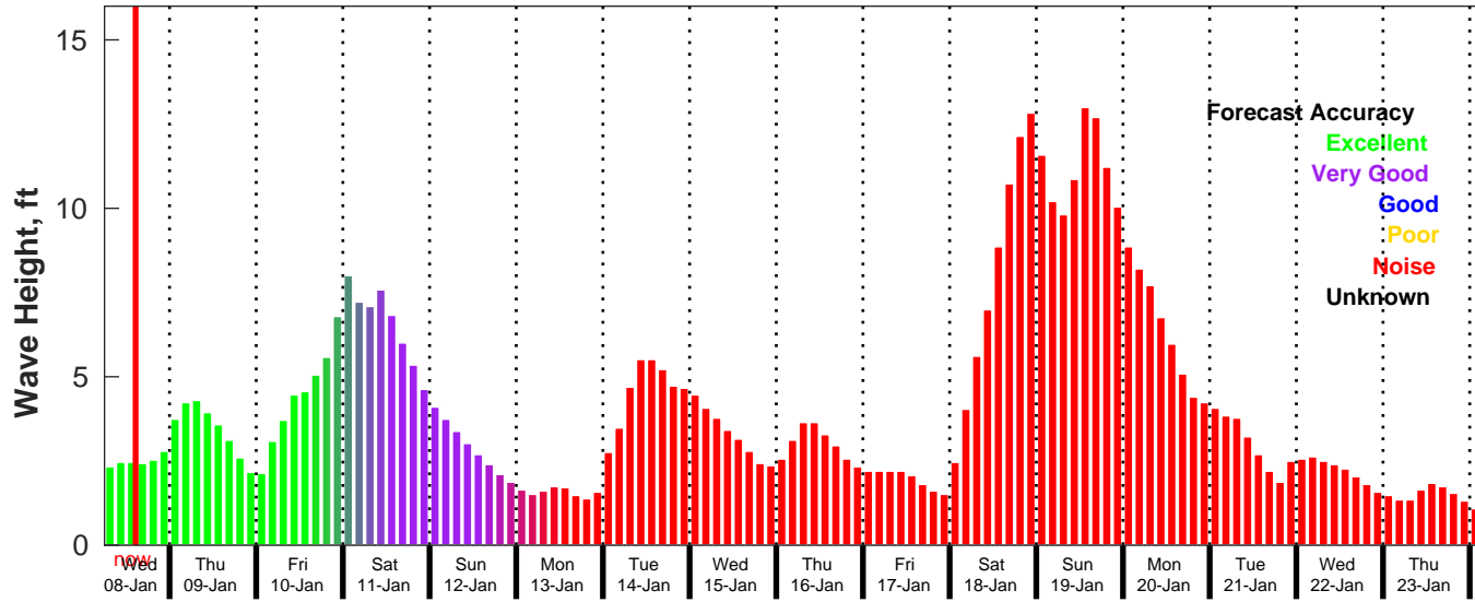
GFS Wave Forecast for NDBC 42036 from 08-Jan-2025 06:00:00 to 24-Jan-2025 06:00:00
