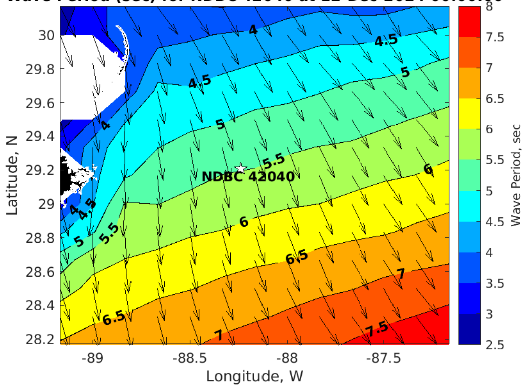
Wave Period (sec) for NDBC 42040 at 12-Dec-2024 00:00:00
