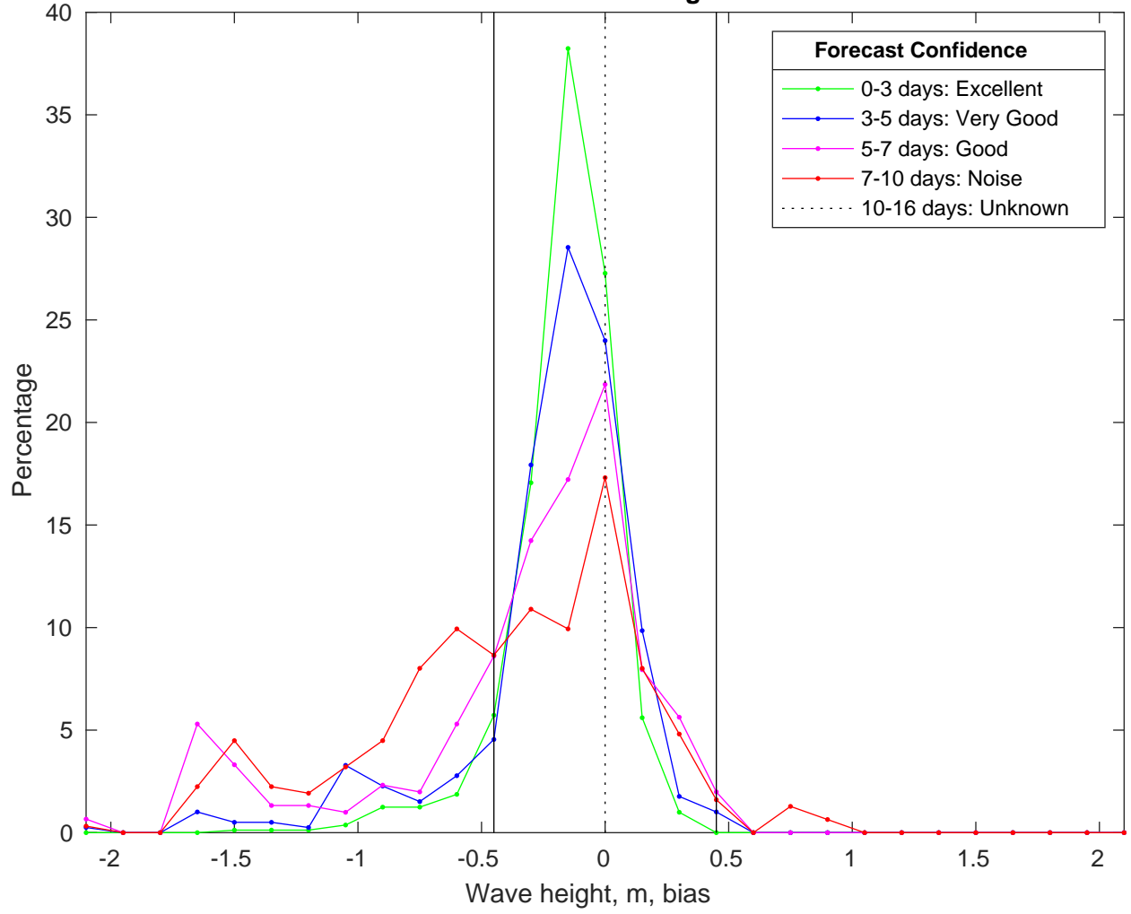
NDBC 42040 vs CMEMSWaves Bias Histogram: 08-Jan-2025
