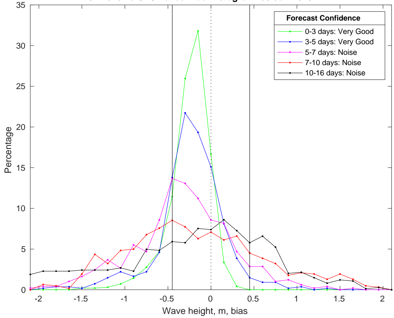
NDBC 42040 vs GFSWaves Bias Histogram: 08-Jan-2025
