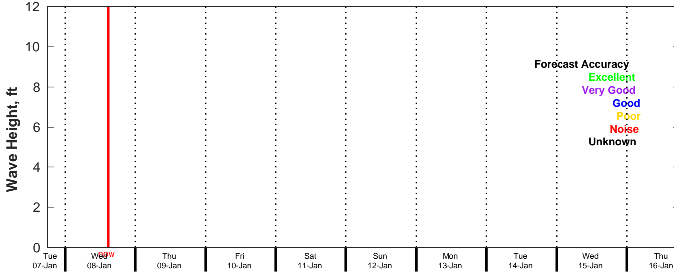
CMEMS Wave Forecast for NDBC 42040 from 07-Jan-2025 18:00:00 to 16-Jan-2025 18:00:00
