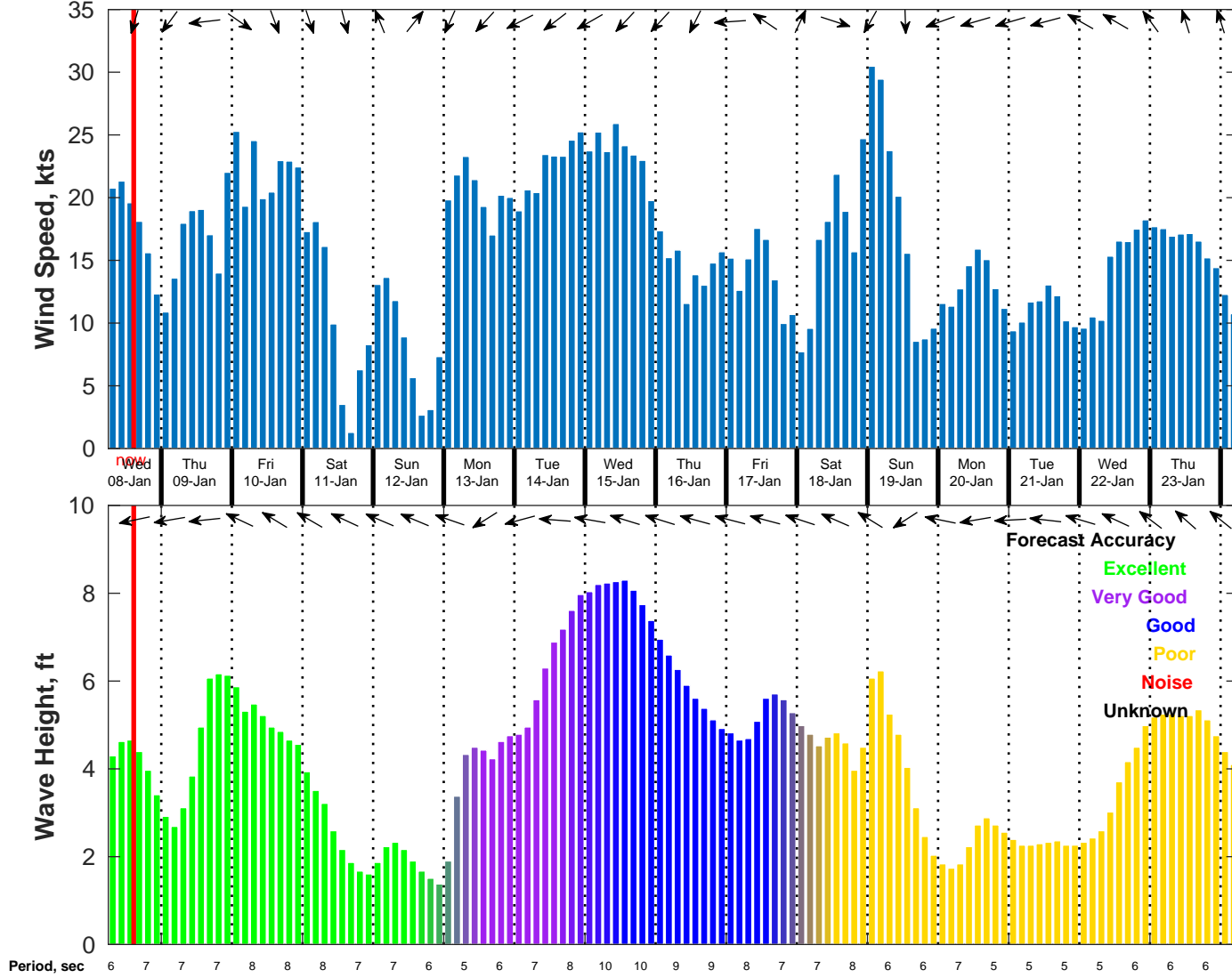
Wind & Wave Forecast for NDBC 42092 from 08-Jan-2025 06:00:00 to 24-Jan-2025 06:00:00
