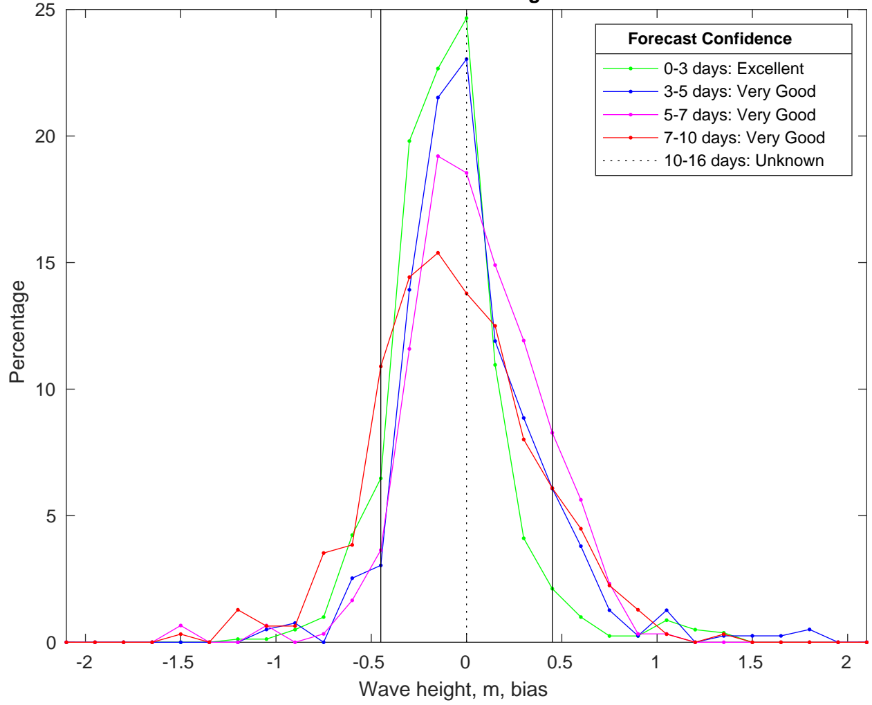
NDBC 46011 vs CMEMSWaves Bias Histogram: 08-Jan-2025
