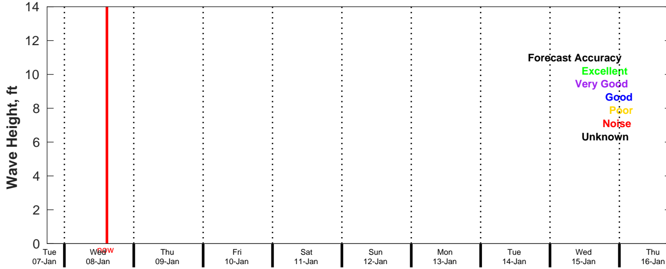
CMEMS Wave Forecast for NDBC 46011 from 07-Jan-2025 18:00:00 to 16-Jan-2025 18:00:00
