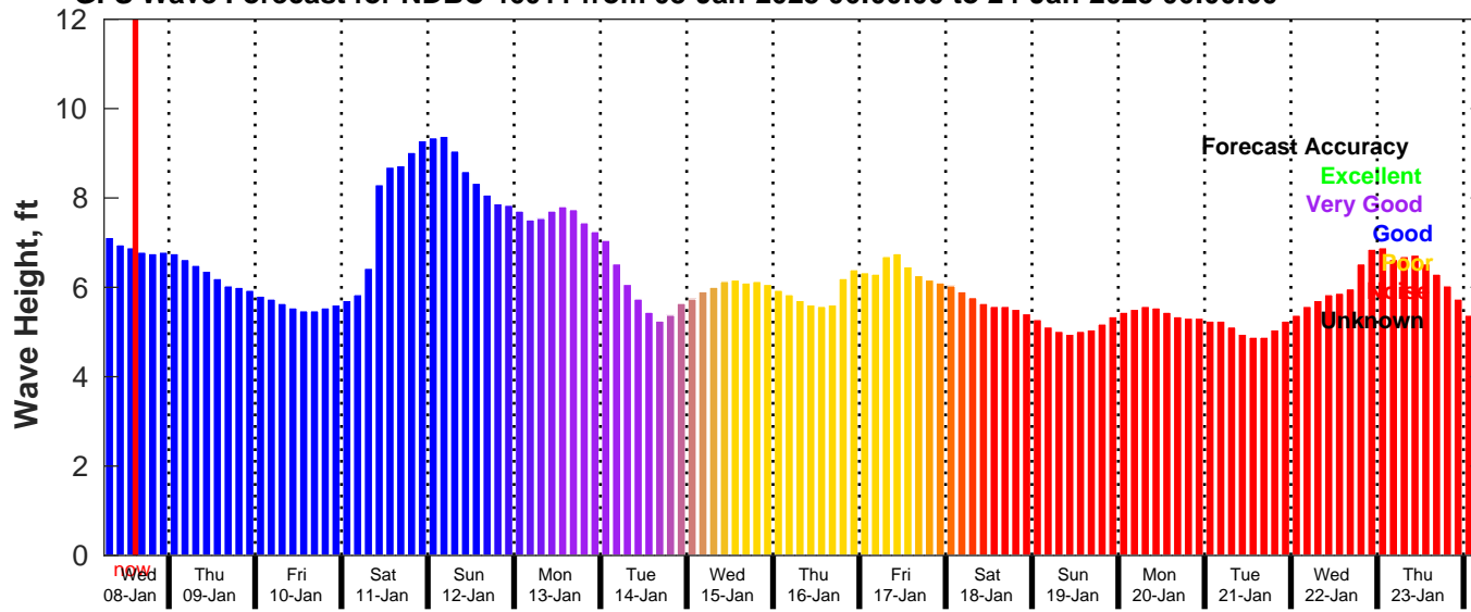
GFS Wave Forecast for NDBC 46011 from 08-Jan-2025 06:00:00 to 24-Jan-2025 06:00:00
