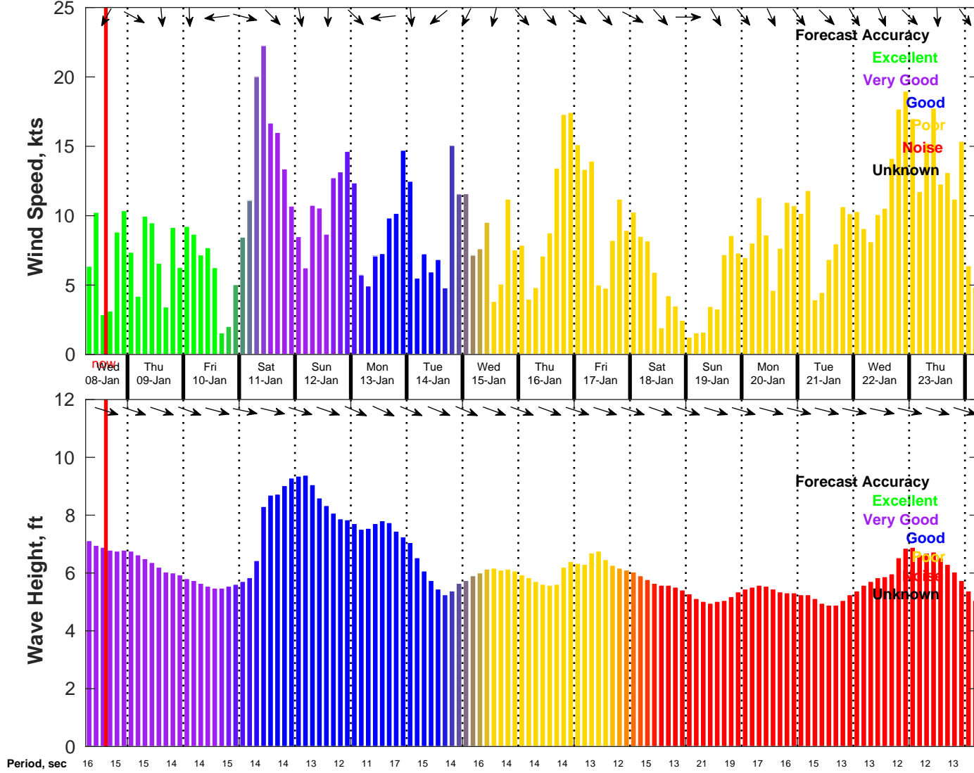
Wind & Wave Forecast for NDBC 46011 from 08-Jan-2025 06:00:00 to 24-Jan-2025 06:00:00
