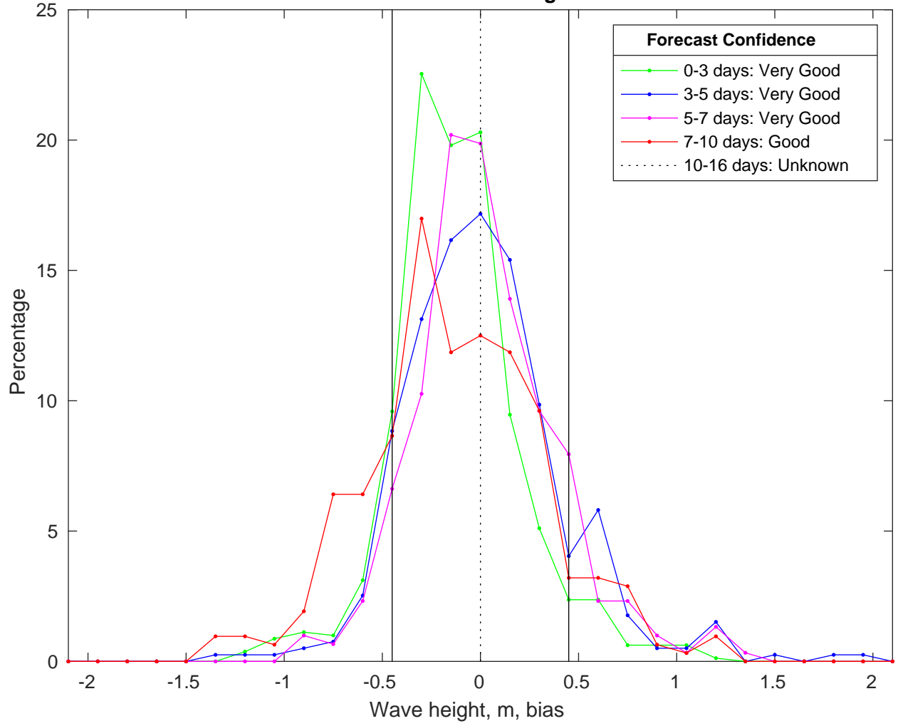
NDBC 46028 vs CMEMSWaves Bias Histogram: 08-Jan-2025
