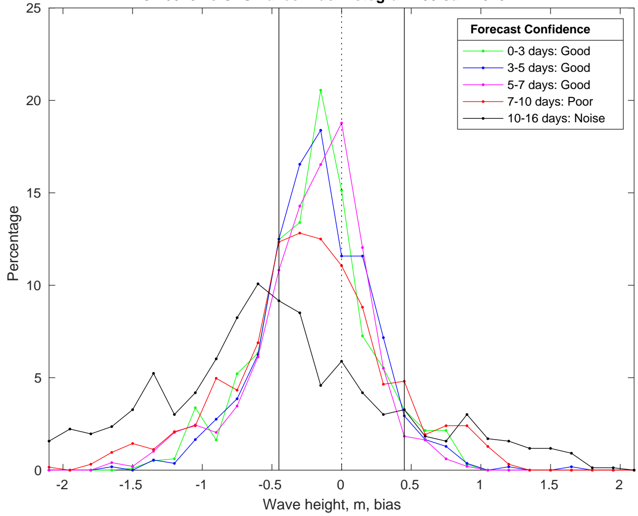
NDBC 46028 vs GFSWaves Bias Histogram: 08-Jan-2025
