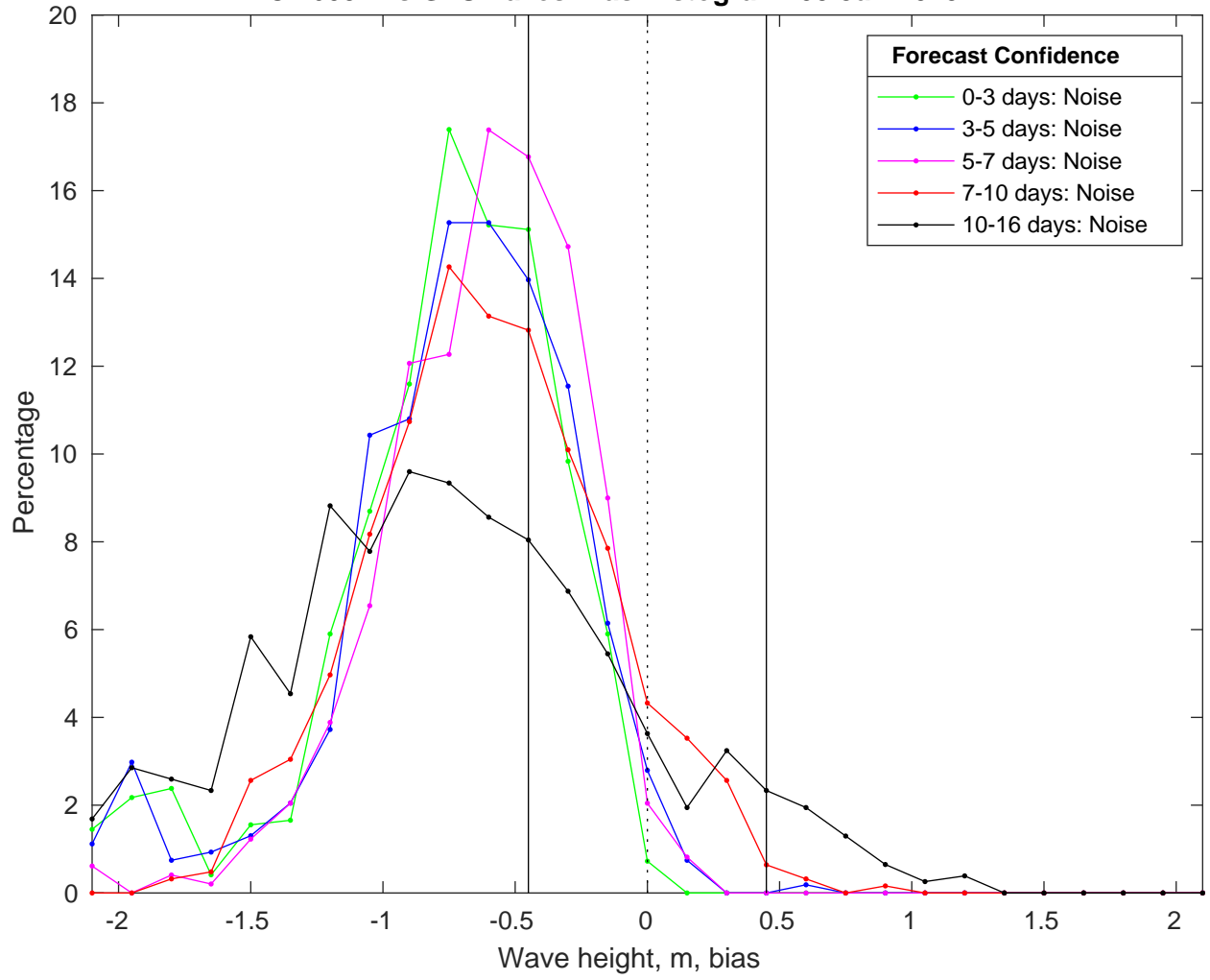
NDBC 46054 vs GFSWaves Bias Histogram: 08-Jan-2025
