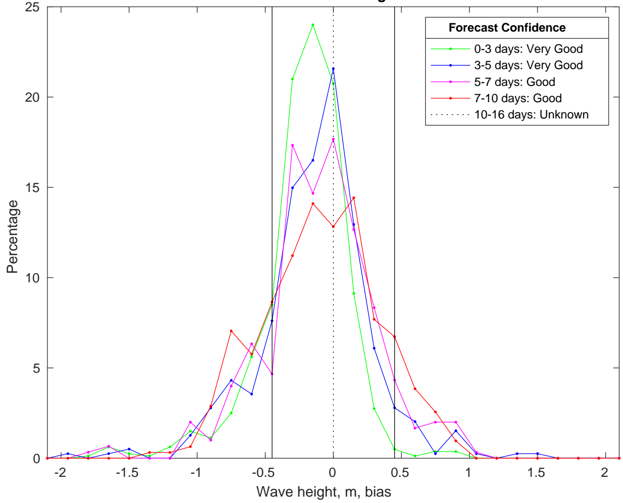
NDBC 46069 vs CMEMSWaves Bias Histogram: 08-Jan-2025
