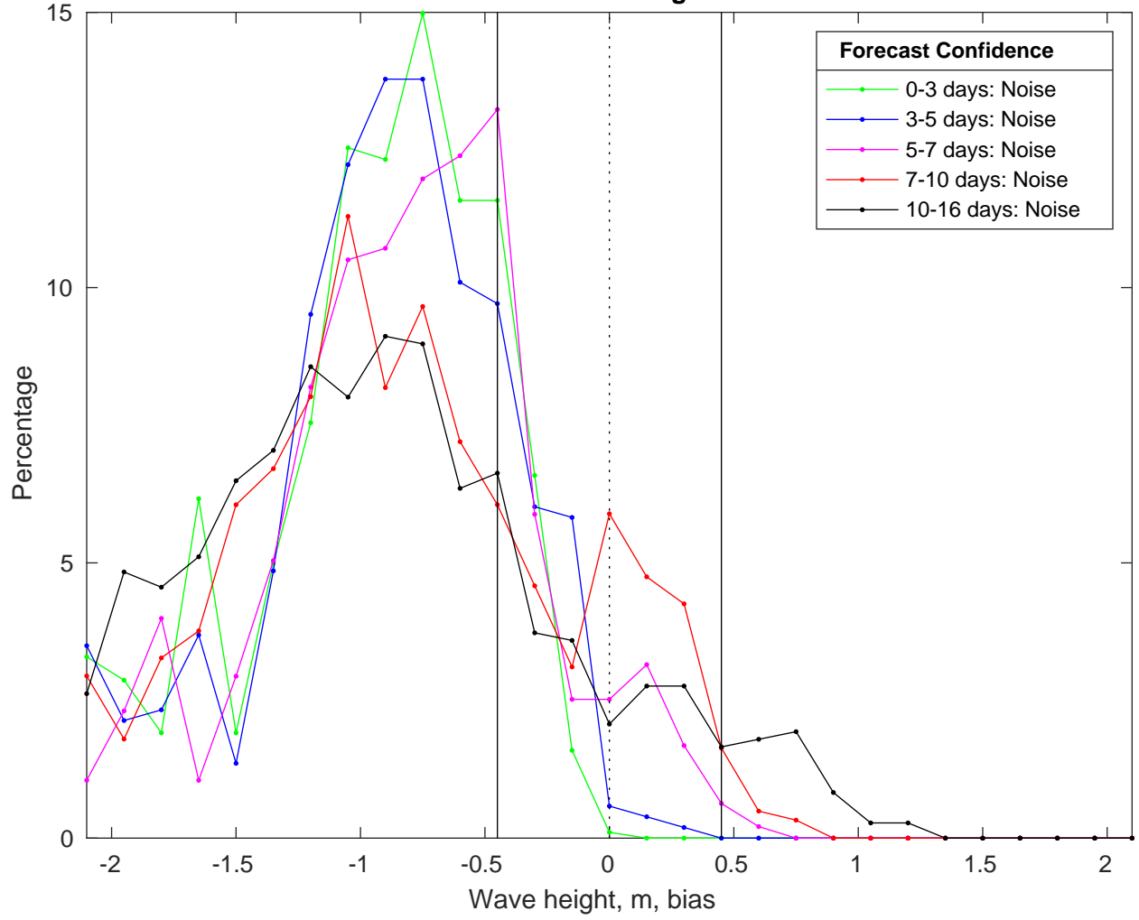
NDBC 46069 vs GFSWaves Bias Histogram: 08-Jan-2025
